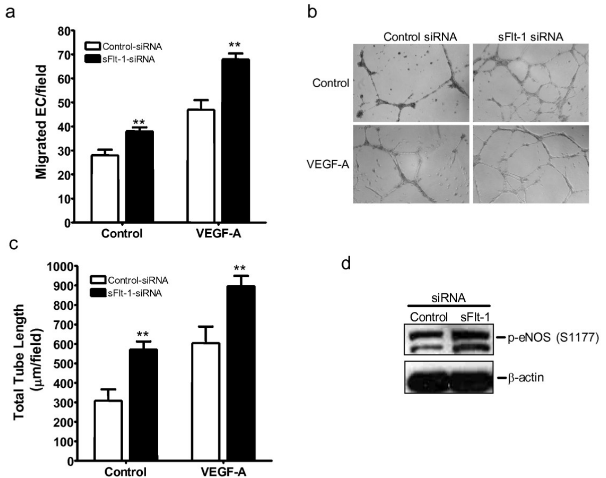
Loss of sFlt-1 enhances angiogenesis and eNOS phosphorylation. (a) VEGF (20 ng/ml) induced an increase in cell migration of HUVEC transfected with sFlt-1 siRNA compared with control siRNA using a modified Boyden chamber assay. (b) VEGF-induced capillary-like tube formation and (c) quantification of mean total tube length per field of view after six hours treatment in HUVEC transfected with sFlt-1 siRNA or control. (d) Representative Western blot showing eNOS phosphorylation at serine 1177 (p-eNOS (S1177)) in HUVEC transfected with soluble (sFlt-1) or control siRNA. β-actin was used as a loading control. Data are expressed as mean (± SEM) or representative of three or more independent experiments performed in triplicate. ** P < 0.01 vs. control.
