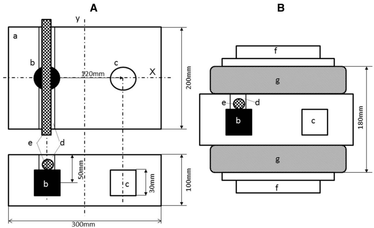
Experimental setup. Schemas of the agar phantom (A) and with the electrode setting (B): a: Agar phantom, b: cylindrical magnetite piece, c: control piece without magnetite, d: groove prepared for setting a blood vessel, e: vessel, f: electrode, g: water cooling pad. The cylindrical magnetite and control pieces were symmetrically placed against the y-axis on the central axis of the agar phantom. A groove was made parallel to the y-axis, and a blood vessel was placed in contact with the cylindrical magnetite piece.
